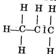
Propene
