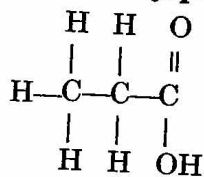
Propanoic acid
