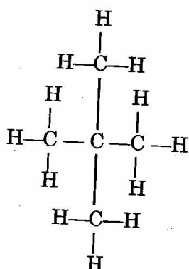
2, 2-dimethylpropane
